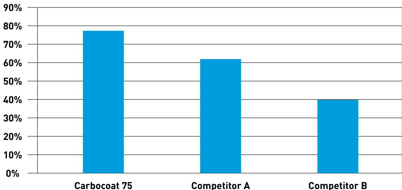
% Gloss Retention at 240 Hours Per ASTM D4587 Fluorescent UV-Condensation
